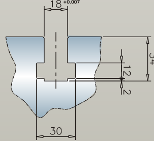
MV-1200 T-slot dimensions
