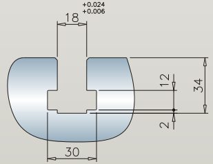
MV-1000 T-slot dimensions
